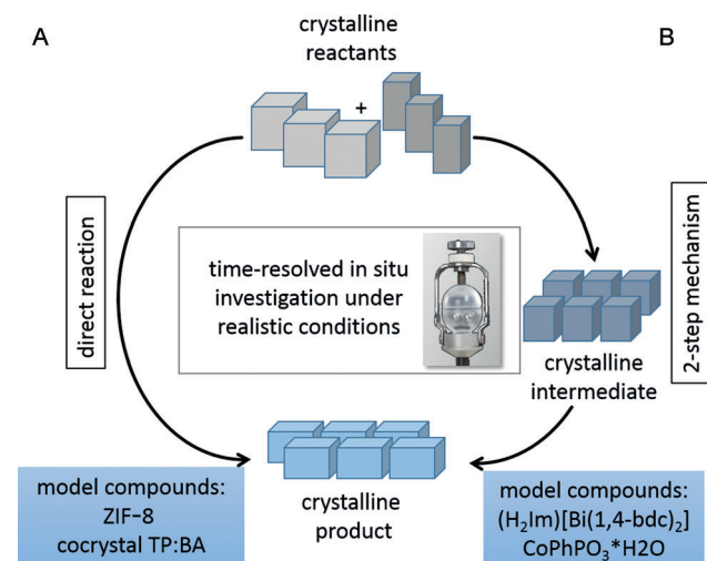
Figure 5. Schematic representation of the two observed synthesis pathways (A and B) indicating an either A) direct conversion or B) a two-step process including a crystalline intermediate.
