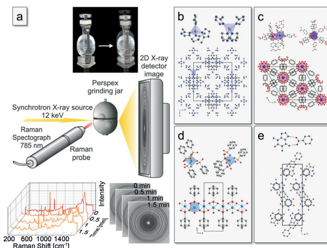
Figure 1. a) Schematic diagram of the experimental setup for collecting Raman spectra and XRD powder patterns during the mechanochemical synthesis. Raman spectra and XRD patterns were typically collected every 30 s. The vibration ball mill is used with 10 mL Perspex grinding jars and two 10 mm stainless steel grinding balls. During the measurements the grinding jar oscillates around the position of measurement. b–e) View of the crystal structures of the investigated metal-organic frameworks ZIF-8 (Zn(Melm) 2 (Melm = 2-methylimidazolate)) 1 and (H 2 Im)[Bi(1,4-bdc) 2 ] (Im = imidazole, bdc = benzenedicarboxylate) 2 , the metal phosphonate cobalt(II) phenylphosphonate monohydrate CoPhPO 3 ·H 2 O (Ph = phenyl) 3 , and the cocrystal theophylline:benzoic acid (1:1) 4 .
